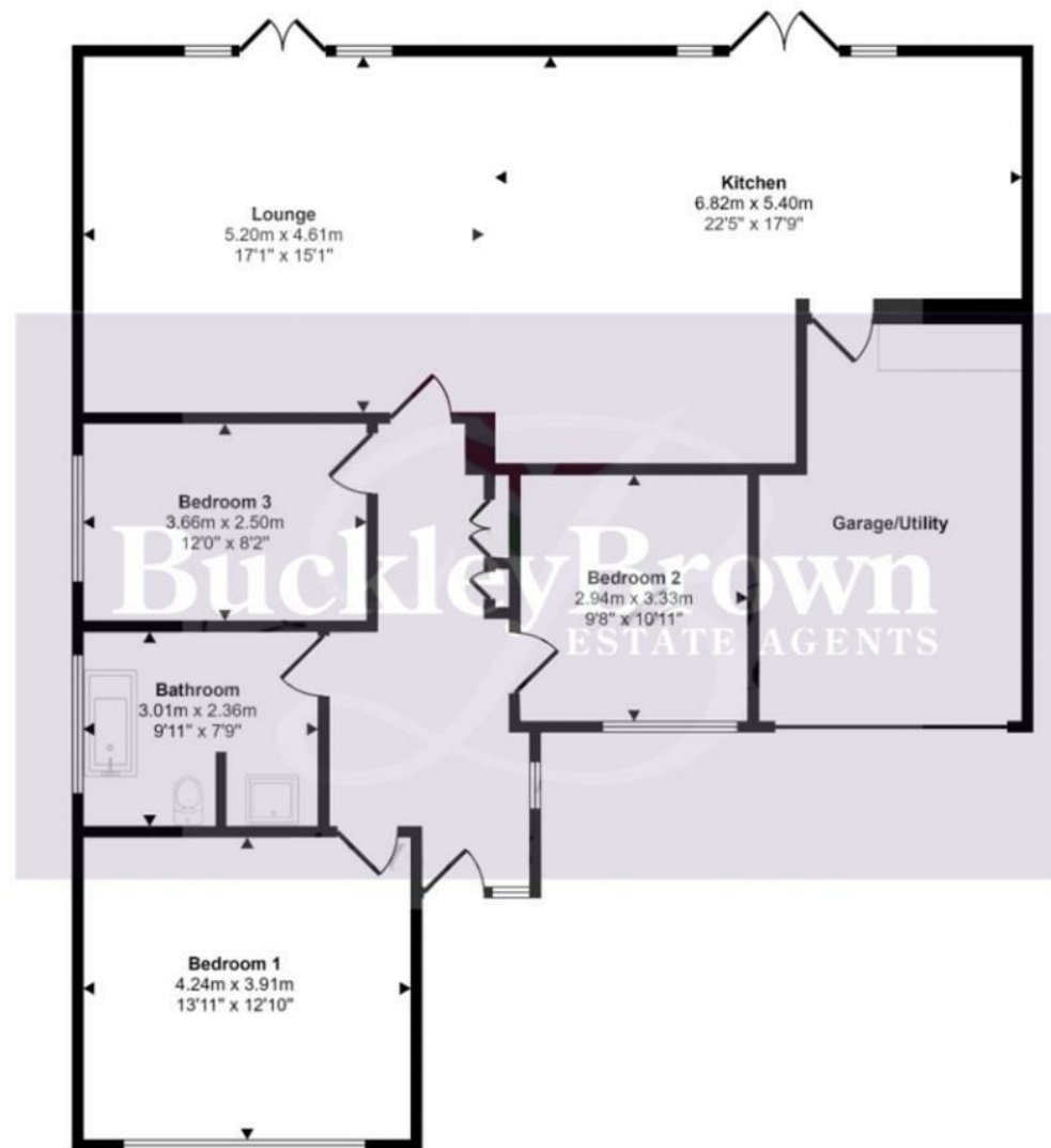
Floorplan
